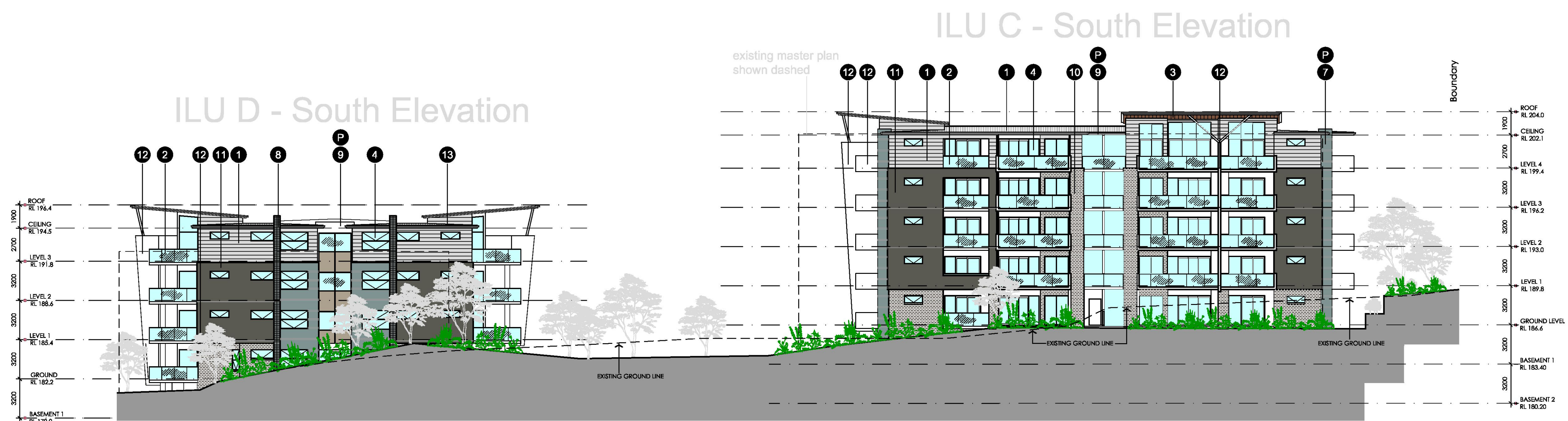
SITE SECTION 8
