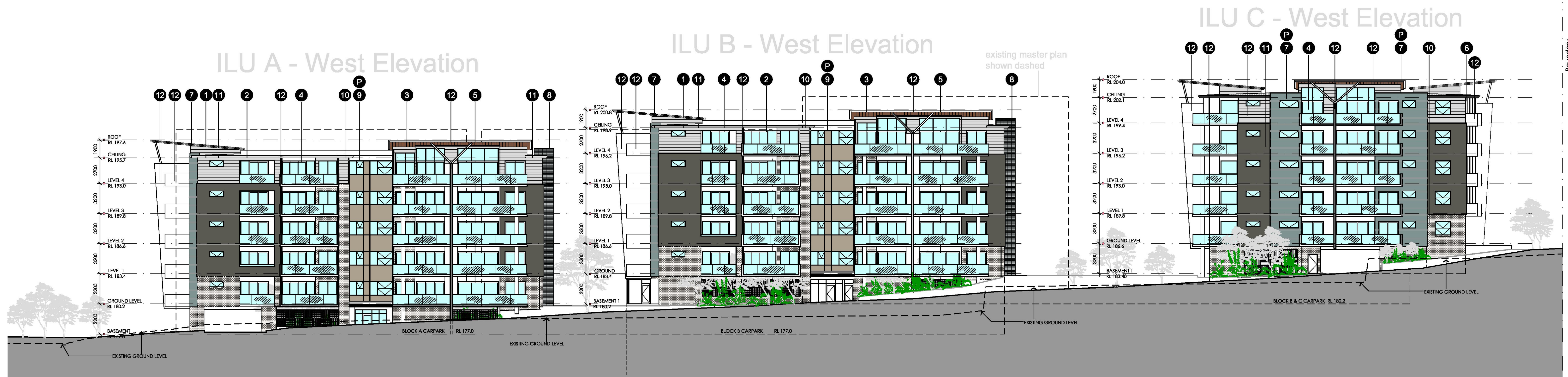
SITE SECTION 1
